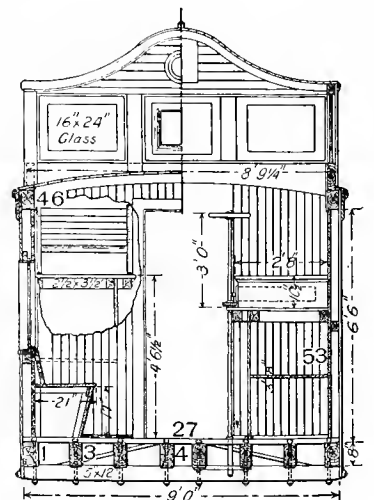
Fig. 384. Half End Elevation.
